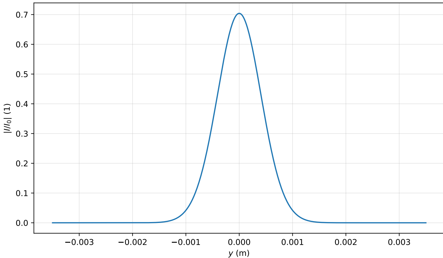
Intensity profile I(x=0, y, z=1.433)/I_0 , P_{in}=0.1P_{cr} , artificial time
